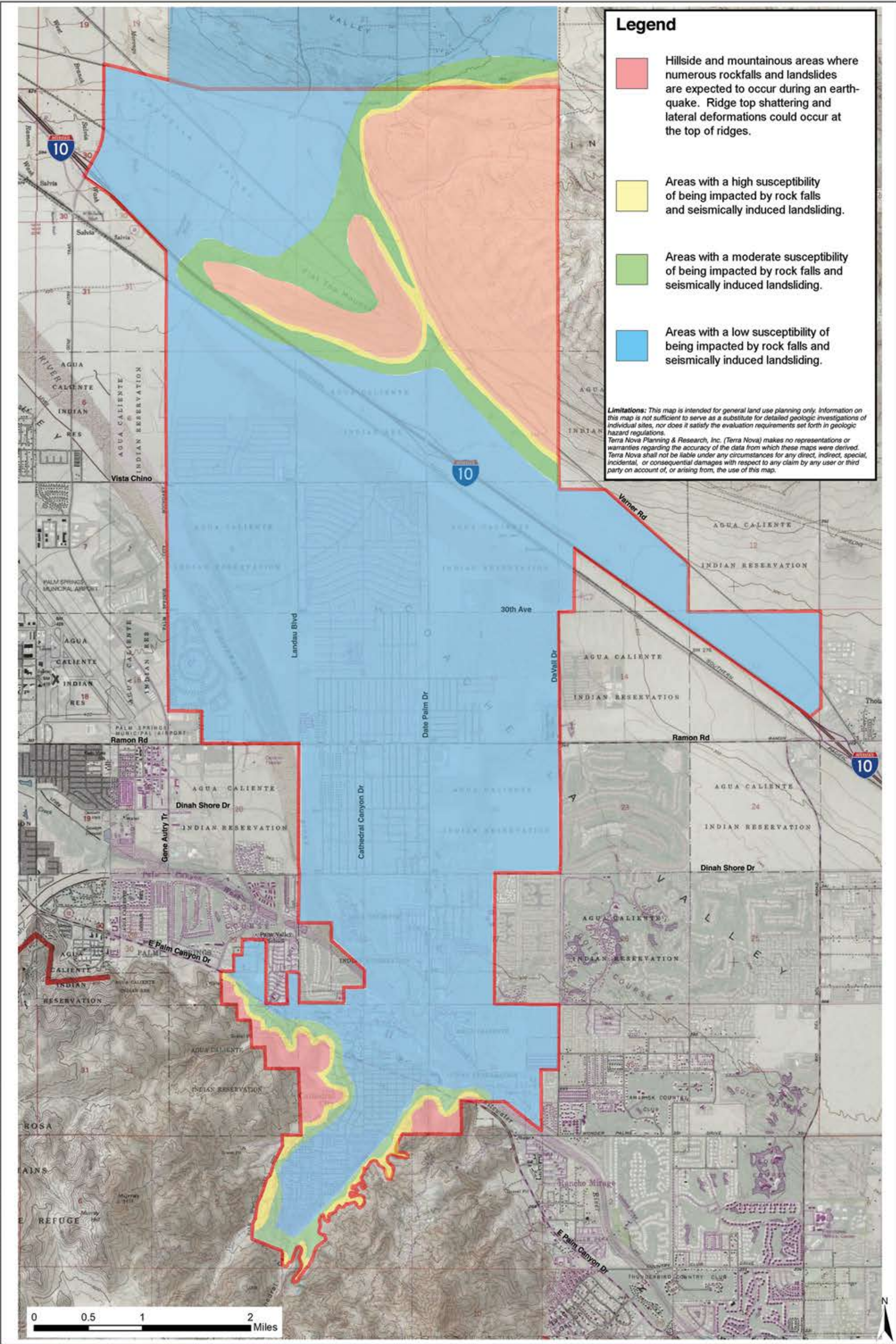
Exhibit S-2 - Seismically Induced Rock Fall and Landslide Suceptibility Cathedral City 2040 General Plan
