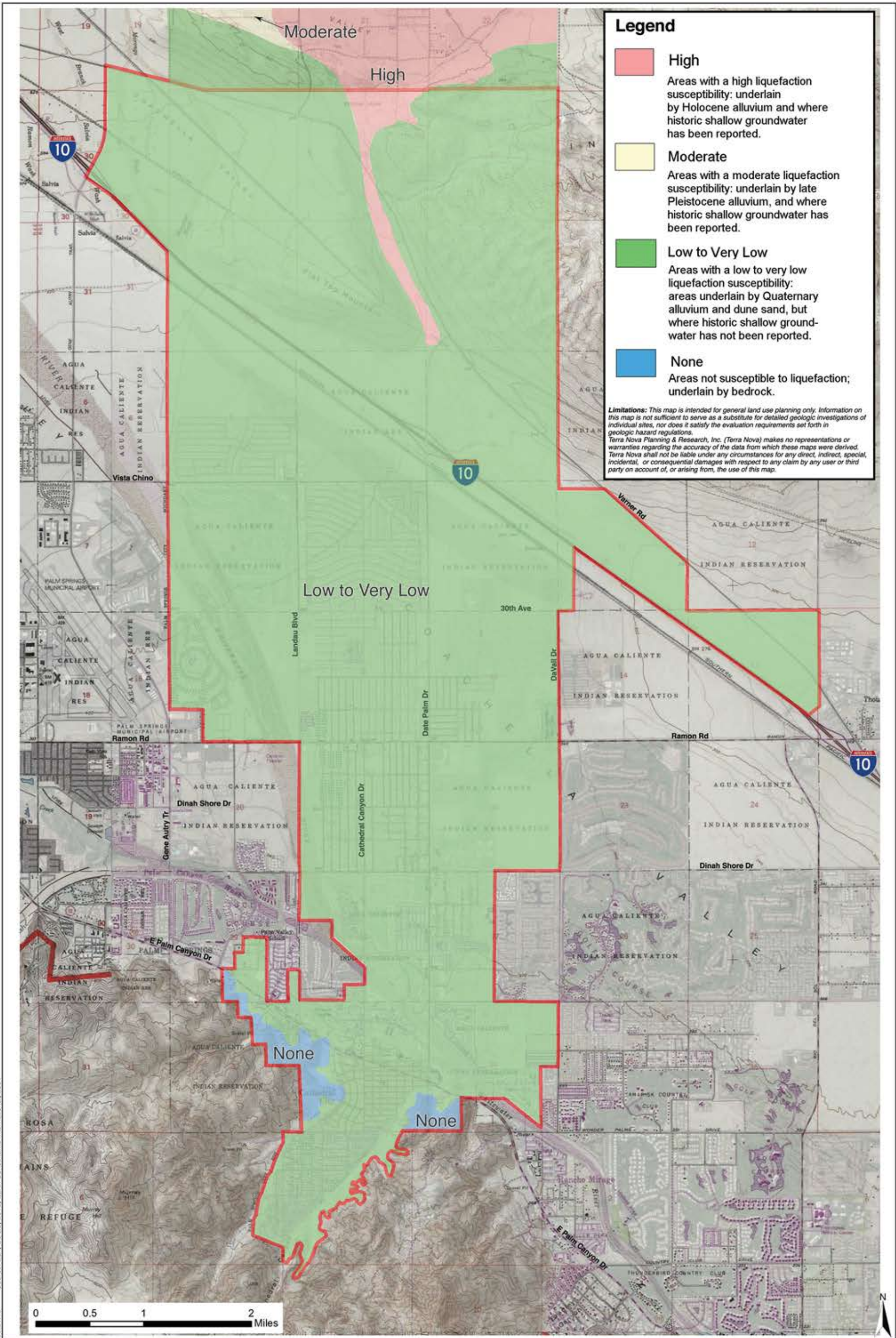
Exhibit S-5 - Liquefaction Suceptibility Map Cathedral City 2040 General Plan
